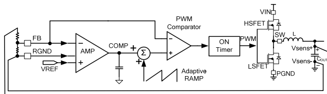
FIGURE 2—COT CONTROL
